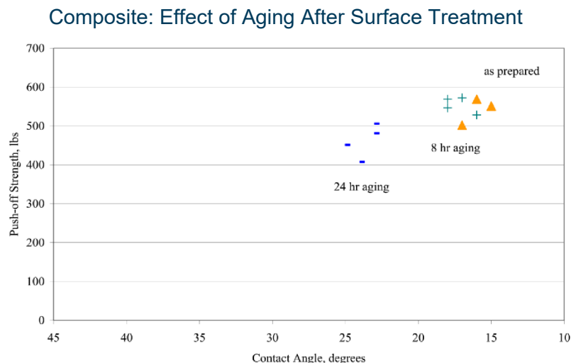
Figure 8. Push off load vs. contact angle for abraded and aged graphite/epoxy substrates.
