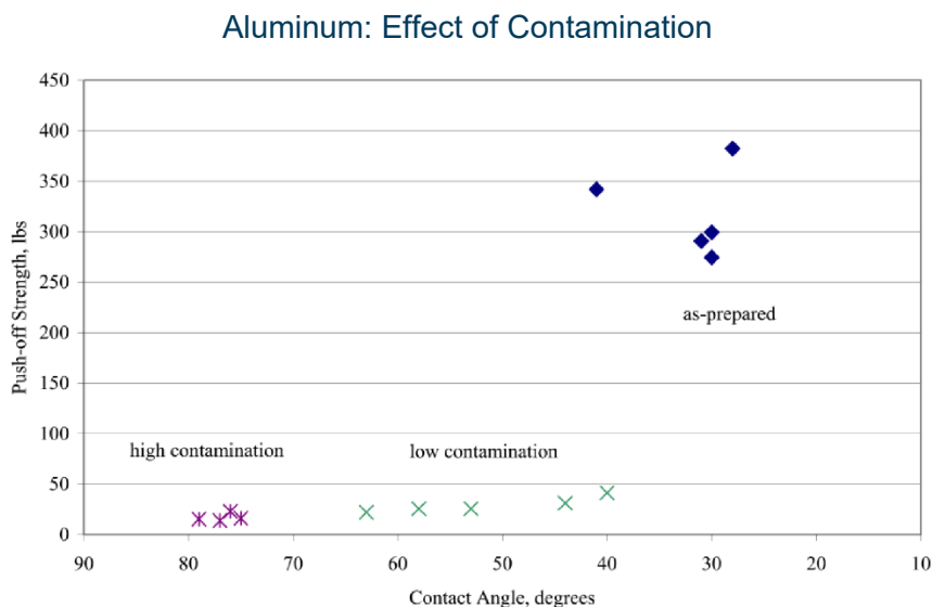
Figure 9. Push-off load vs contact angle for abraded and contaminated Al substrates.
