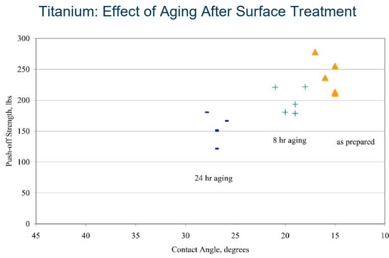
Figure 7. Push-off load vs. contact angle for abraded and aged Ti-6Al, 4V substrates.
