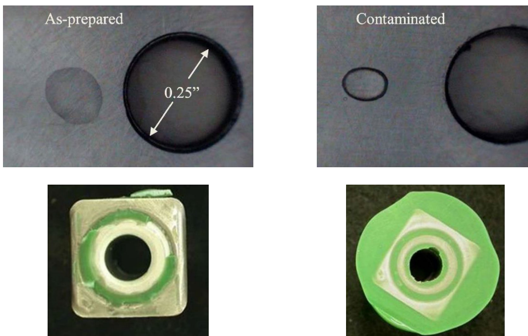
Figure 5. Top: Ti-6Al, 4V surfaces prepared for bonding by abrasion and solvent wiping. Bottom: corresponding nutplate failure surfaces.
