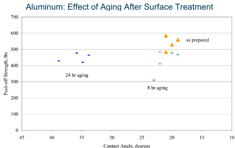
Figure 6. Push off load vs. contact angle for abraded and aged aluminum substrates.
