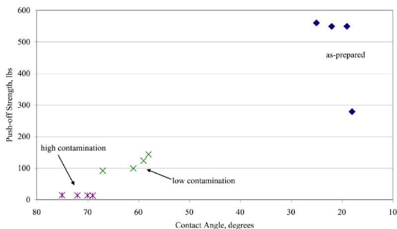
Figure 10. Push-off load vs. contact angle for abraded and contaminated composite substrates.
