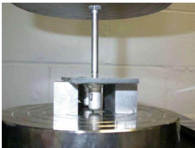
Figure 4: Determination of bond strength of nutplates.
