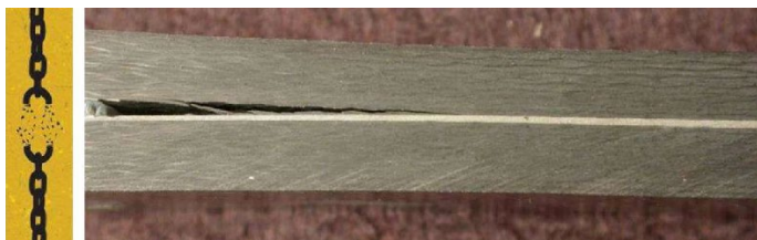
Figure 2: Bonded graphite/epoxy composite loaded to failure in Mode I. Crack propagation is in the composite, the phase with the lowest fracture toughness in this structure.
