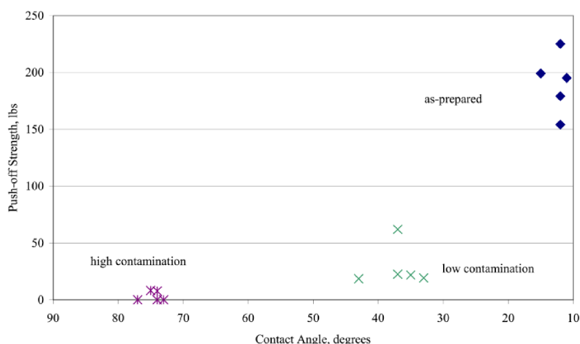
Figure 10. Push-off load vs. contact angle for abraded and contaminated Ti-6Al, 4V substrates.
